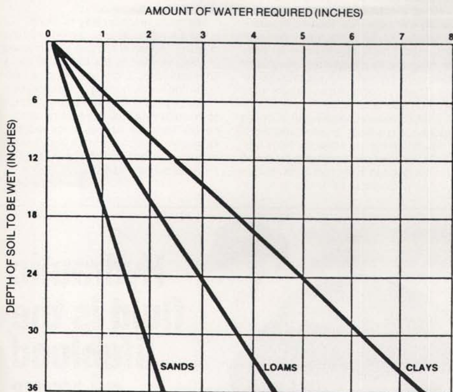
Inches of water required to wet soils to given depths (assuming no runoff).
