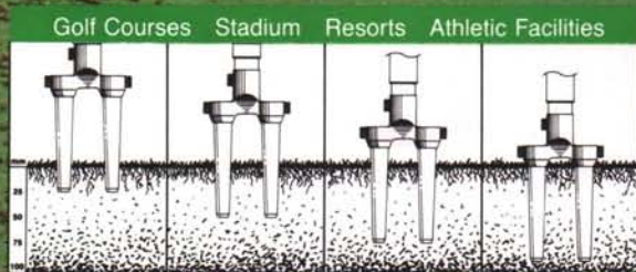
Golf Courses Stadium Resorts Athletic Facilities SHALLOW CORING DE-THATCHES MEDIUM CORING RELIEVES COMPACTION DEEP CORING IMPROVES DRAINAGE VERY DEEP CORING FOR MAJOR RENOVATIONS
